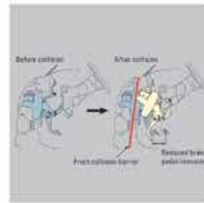
Brake pedal and steering shaft intrusion-reduction system
